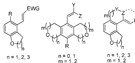
FIGURE 1. Synthesis of benzofurans, dibenzofurans, and dihydrochromenes.
